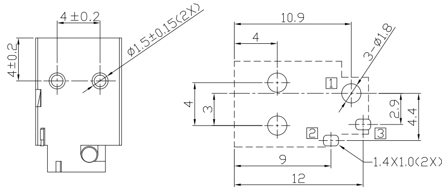
RECOMMENDED P.C.B. LAYOUT UNSPECIFIED TOLERANCE: \pm 0.05 (BOTTOM VIEW)
