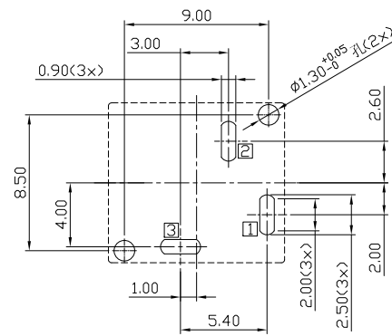
P.C.B LAYOUT (TOLERANCE: ±0.05mm) TOP VIEW (T=1.60mm)
