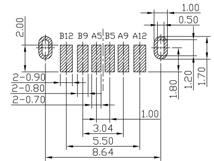
RECOMMEND P.C.B LAYOUT TOLERANCE UNSPECIFIED ±0.05mm
